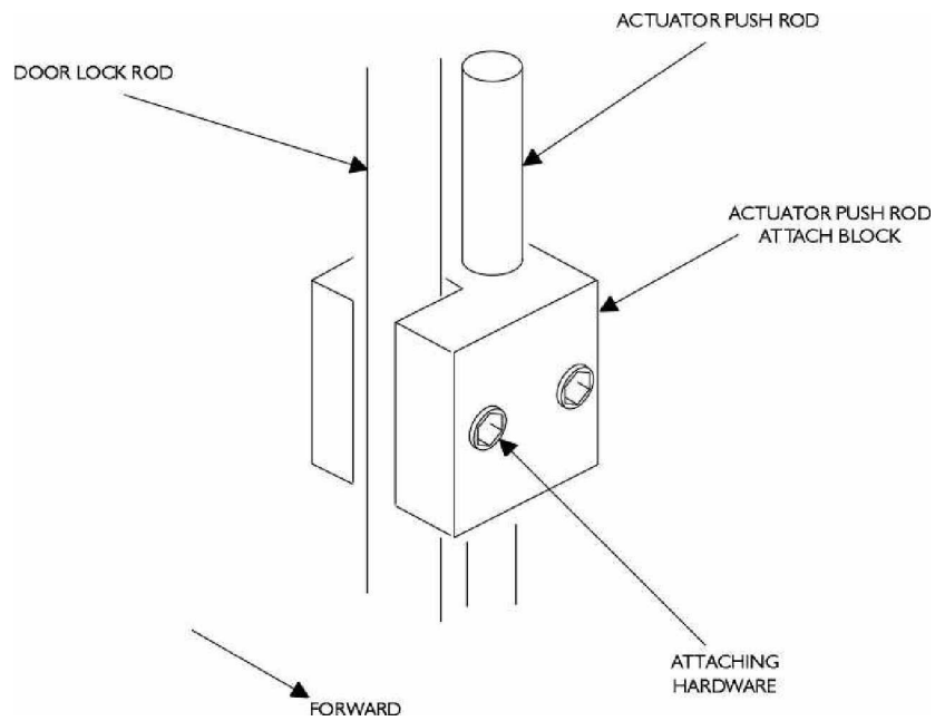
Figure 6. Actuator H block
