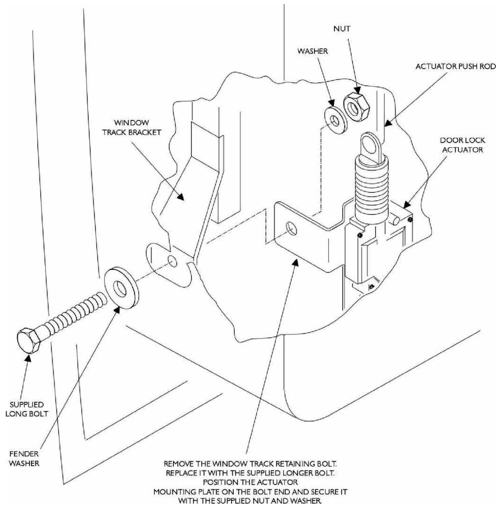
Figure 5. Mounting the actuator to the door.
